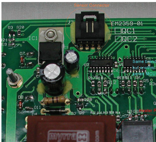
sensor connection
