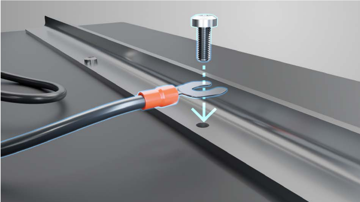
11. Ground the installation niche The installation niche needs to be connected to the pool grounding on the top of the niche.
