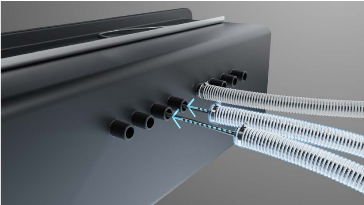
12. Mount the conduit pipes The cables need to be placed in separate conduit pipes.
